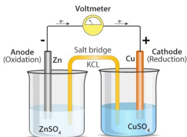
Daniel Cell
