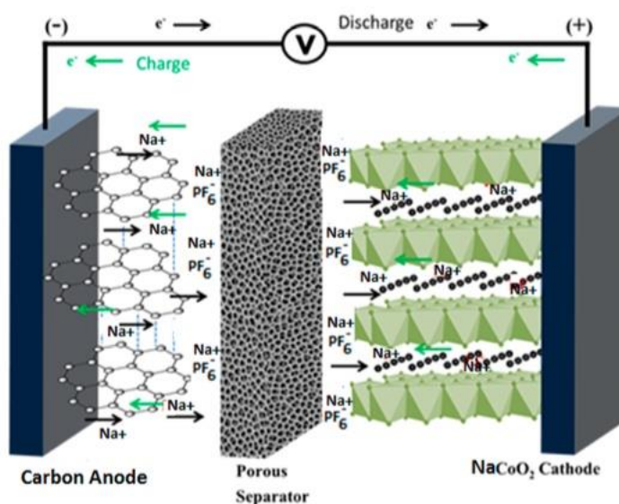
Na-ion Battery
