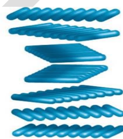
Cholesteric phase
