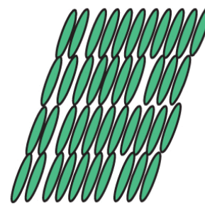
Smectic C
